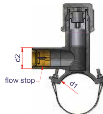
* gas stop in ottone brass device
