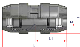
MANICOTTO COUPLER
