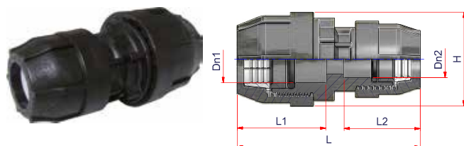
MANICOTTO RIDOTTO REDUCING COUPLER
