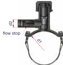
• gas stop in plastica plastic device
