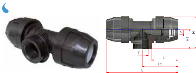
TEE 90° FILETTATO FEMMINA 90° TEE WITH FEMALE OFFTAKE
