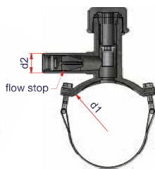
• gas stop in plastica plastic device
