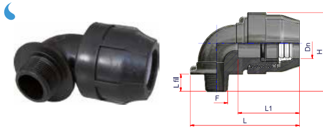
GOMITO A 90° FILETTATO MASCHIO 90° ELBOW WITH MALE OFFTAKE
