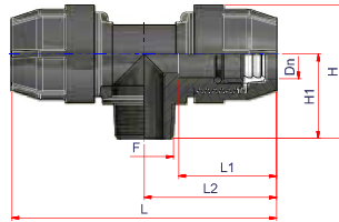
TEE 90° FILETTATO MASCHIO 90° TEE WITH MALE OFFTAKE
