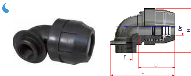
GOMITO A 90° FILETTATO FEMMINA 90° ELBOW WITH FEMALE OFFTAKE
